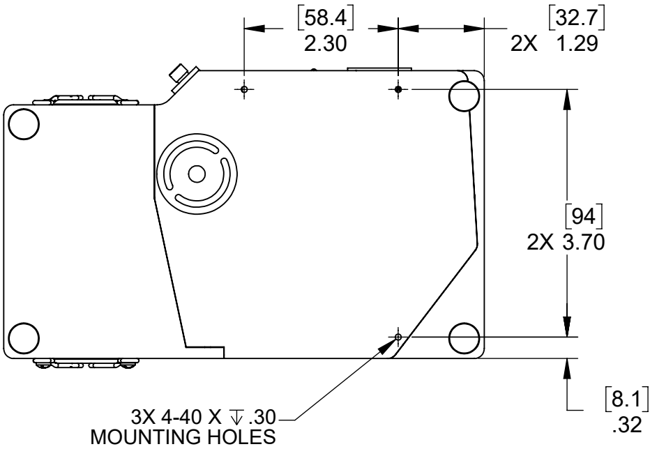
BOTTOM VIEW
